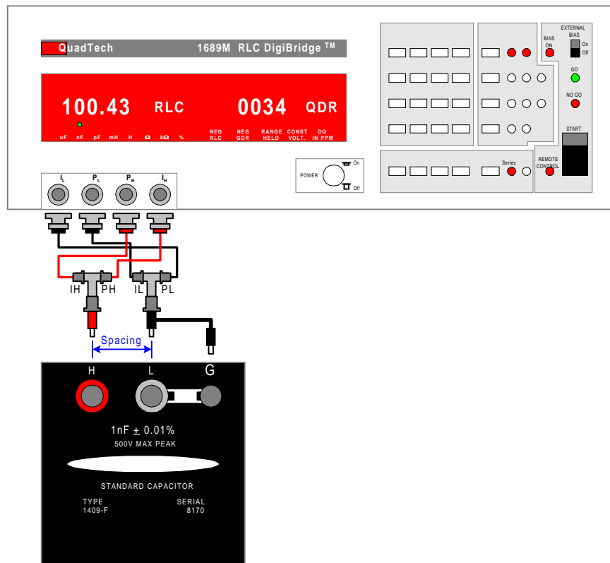
Figure 1: 1689M DigiBridge connected to 1409 Capacitor Standard
